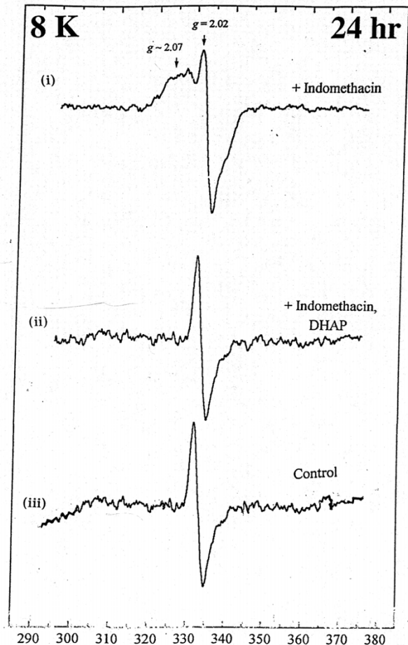
Figure 5 Comparison of EPR spectra of indomethacin and DAHP pre-treated indomethacin group at 8 K after 24 hr treatment.
