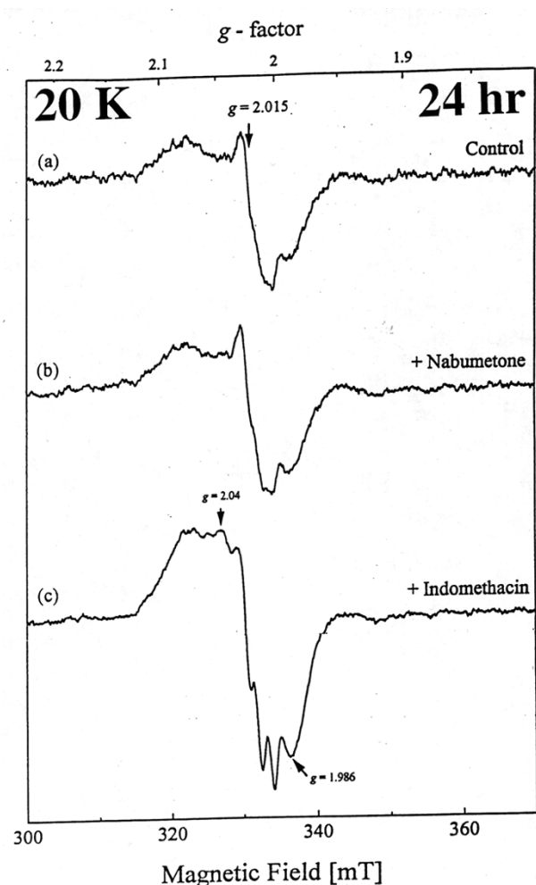
Figure 3 The EPR spectra of rat jejunal homogenates at 20 K after 24 hr oral gavage of (a) DMSO, (b) nabumetone (500 mg / kg b.wt) and (c) indomethacin (20 mg/kg b.wt)
