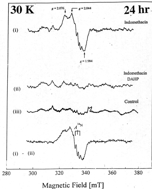
Figure 4 Comparison of EPR spectra of indomethacin and DAHP pre-treated indomethacin group at 30 K after 24 hr treatment.
