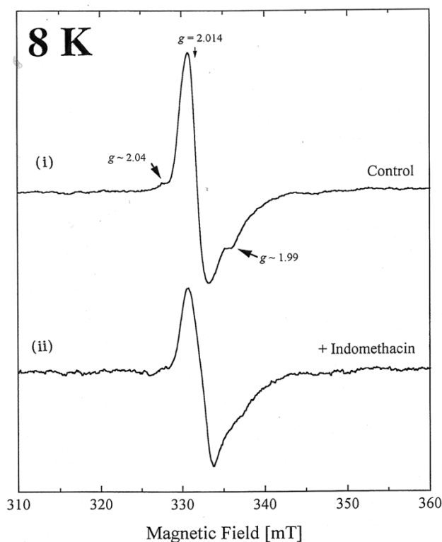
Figure 1 The EPR spectra of (i) DMSO-control and (ii) indomethacin (25 mM final concentration) treated bovine heart sub-mitochondrial particles at 8 K.
