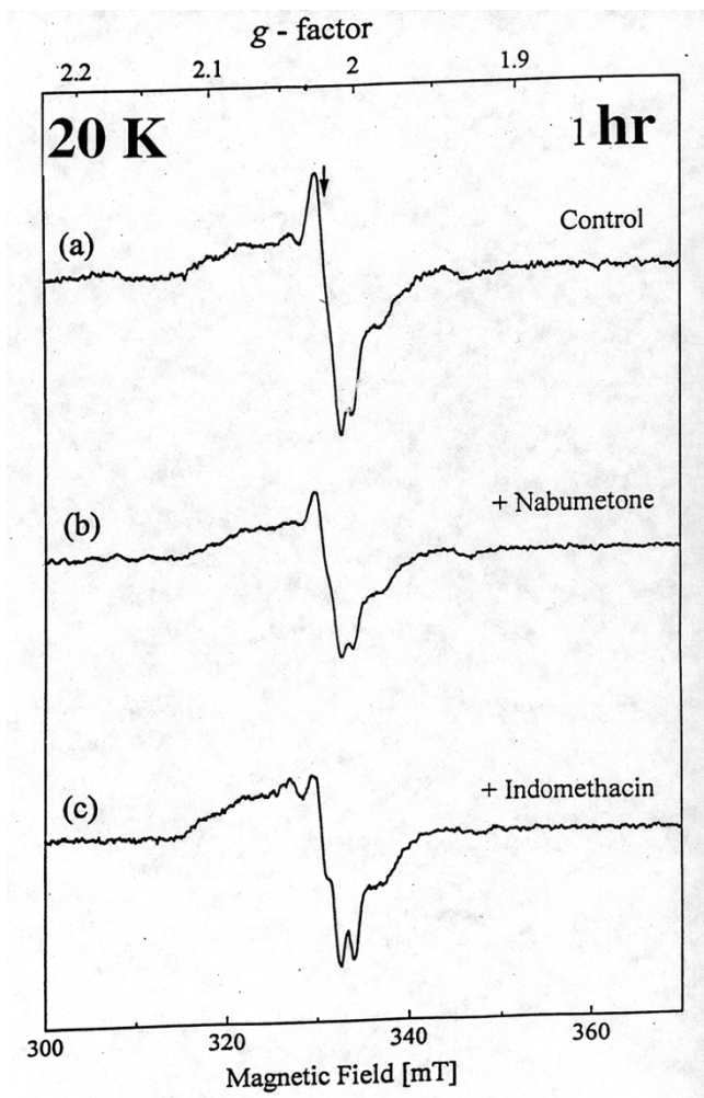
Figure 2 The EPR spectra of rat jejunal homogenates at 20 K after 1 hr oral gavage of (a) DMSO, (b) nabumetone (500 mg / kg b.wt) and (c) indomethacin (20 mg/kg b.wt)
